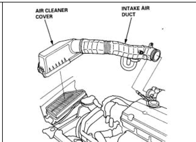
Fig 2: Removing stock air duct
