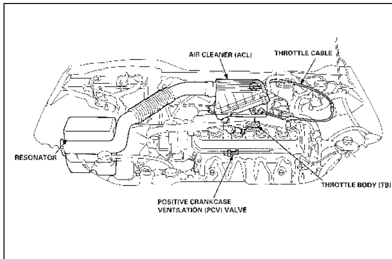
Fig.3: Air inlet layout
