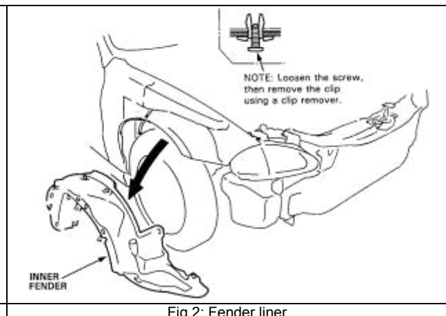
Fig.2: Fender liner
