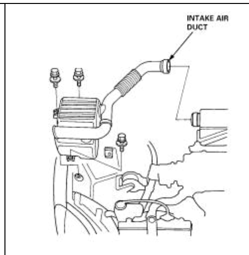
Fig.4: Removing air inlet resonator
