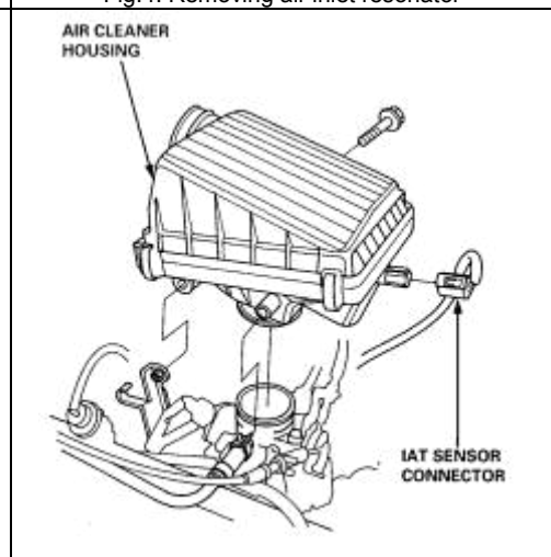
Fig.6: Removing air filter case
