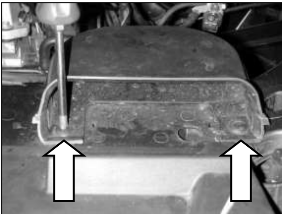
m. Remove the two bolts securing the air inlet duct from the vehicle.
