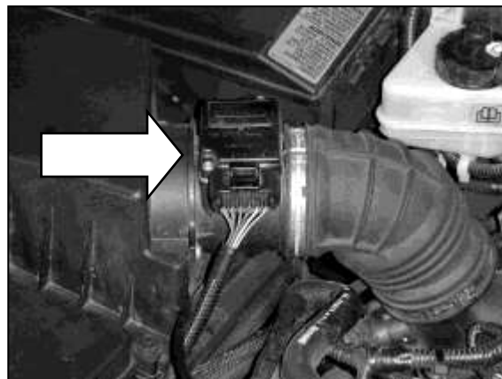
b. Remove the wiring harness from the MAF Sensor.
