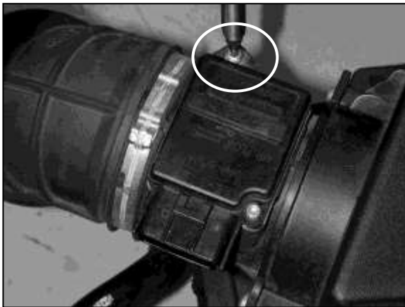
g. Remove the MAF sensor from the factory inlet tube.
