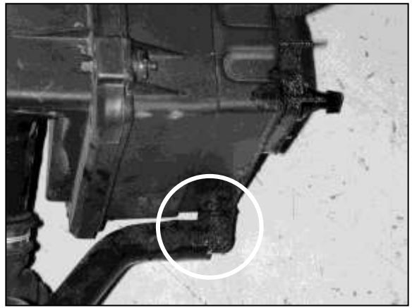
h. Remove the 90 degree plastic fitting from the air box assembly.
