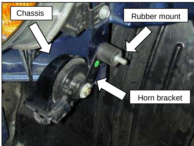
d. Install 8mm rubber mount through horn bracket into the chassis.
