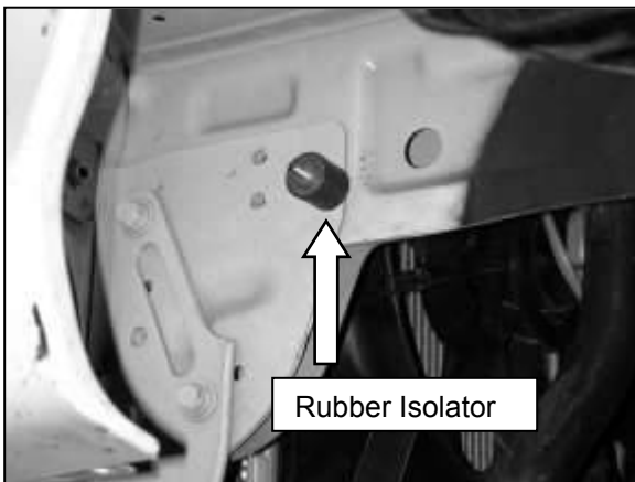
b. Install the included rubber isolator in the factory threaded hole in the frame rail, as shown.
