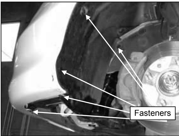
e. Remove the fasteners holding the front inner fender liner, and flex it back for access.
