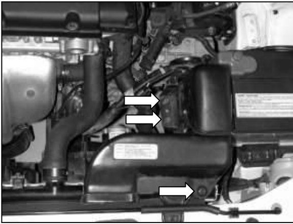
c. Loosen the three bolts holding the cool air duct to the body; then remove it.
