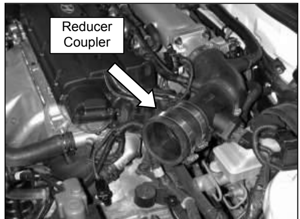
c. Install the included reducer coupler onto the MAF sensor, and secure it with the supplied No. 44 hose clamp.
