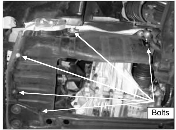
d. Loosen the 5 bolts securing the inner splash panel to the frame rail, and remove it.
