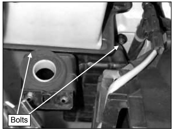
f. Loosen the two bolts holding the resonator box, and remove it.
