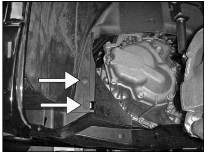
d. Remove one (1) screw and one (1) pop grommet from the splash guard.
