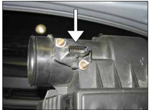
e. Loosen and remove the MAF Sensor mounting bolts and sensor from the air box.
