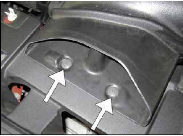
af. Re-install the plastic retaining clips to secure the inlet of the intake scoop.
