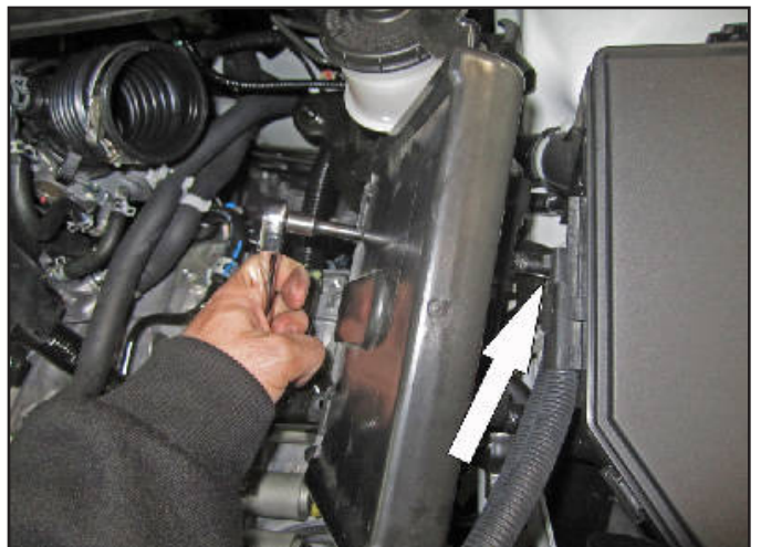
n. Move the ECU to gain access to the remaining 10mm bracket bolt. Remove bolt.
