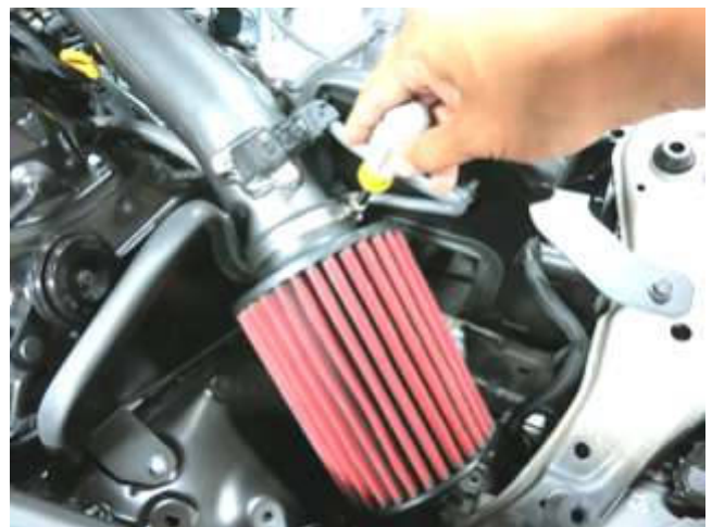
j. Install the AEM filter onto the inlet end of the tube. Adjust for clearance and secure down with the provided hose clamp(9452).
