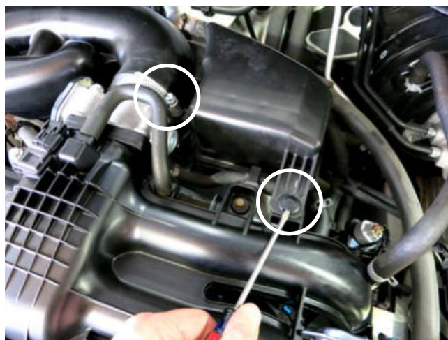
b. Remove the clip securing the stock intake resonator to the engine. Then loosen the hose clamp at the throttle body.
