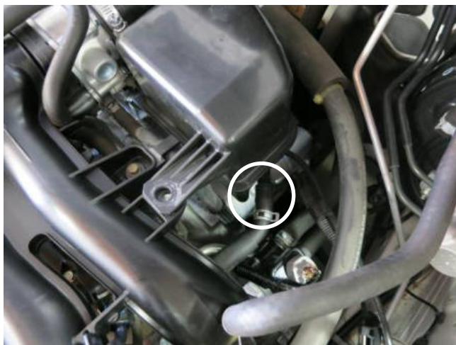
c. Release the pressure on the spring clamp and remove the vent hose underneath the resonator.
