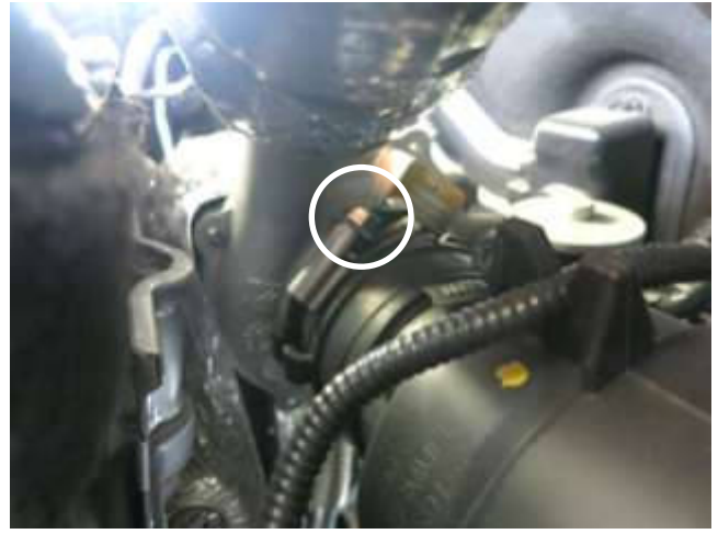
f. Loosen the hose clamp at the turbo compressor.
