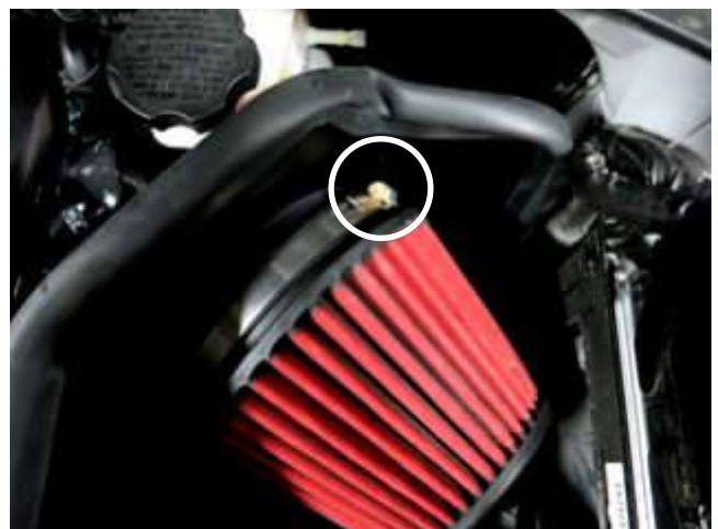
p. Install the AEM filter onto the filter adaptor and tighten the hose clamp.
