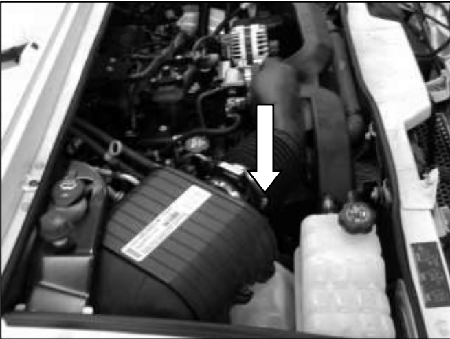
a. Loosen hose clamp on the MAF side of the inlet hose.
