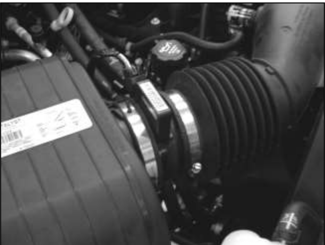
c. Loosen the hose clamp connecting the MAF sensor to the air box.
