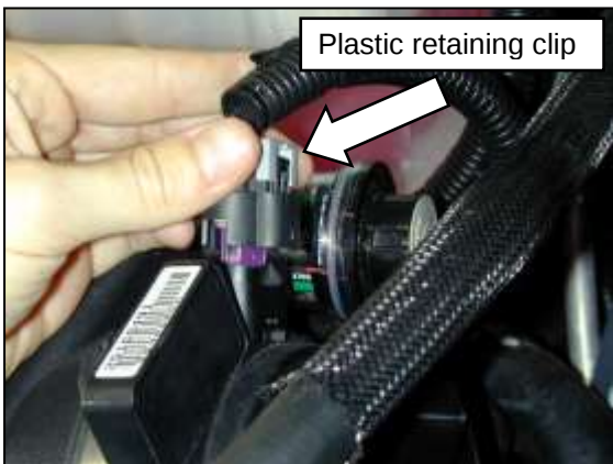
c. Pull back the plastic retaining clip and disconnect the MAF sensor wire harness connector.
