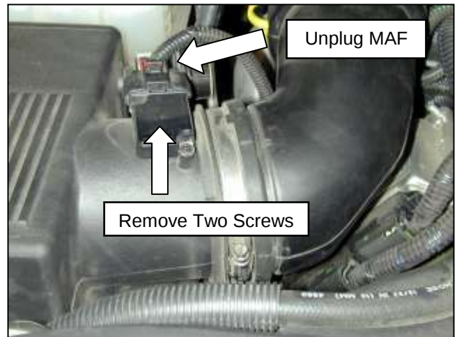
b. Unplug the wire harness from the mass air flow (MAF) sensor. Remove the two screws retaining the MAF sensor with the supplied torx tool. Carefully remove the MAF sensor.
