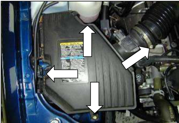
c. Loosen the hose clamp on the stock air box. Remove the air box by removing the two bolts and the nut securing it. Lift air box out of vehicle.
