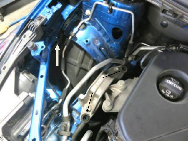
g. Ensure the two rubber grommets in the engine mount are still installed. If they have been removed with the air box, reinstall them at this time. The third rubber grommet located along the inner fender (denoted by the white arrow) will not be reused and can be kept on the air box.
