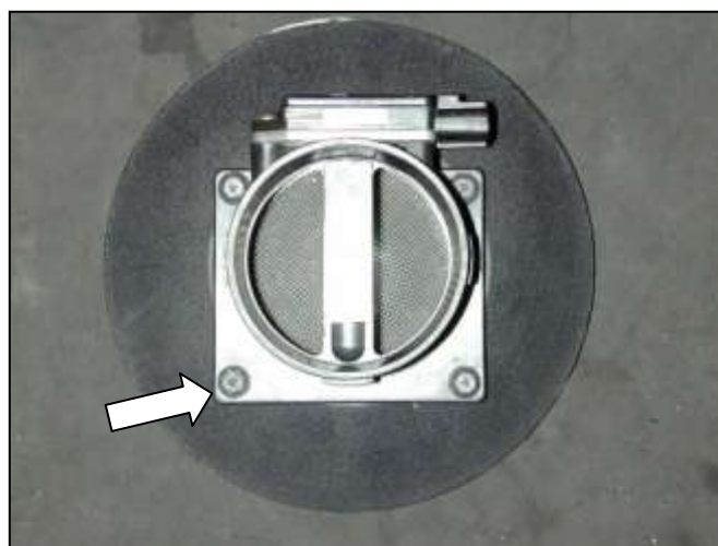
f. Loosen and remove the 4 bolts retaining the MAF sensor. Remove the MAF sensor. The screen will not be reused.
