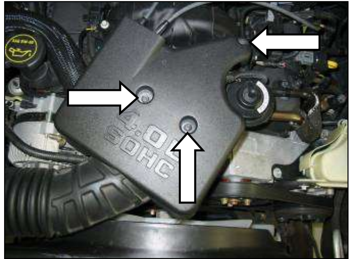
b. Remove the three screws that secure the throttle body cover. Remove the throttle body cover.
