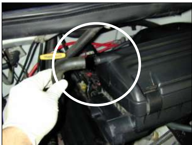
c. Remove the crankcase breather hose from the air filter housing. If the hose is on the passenger side of the air box, the hose may be left connected to the valve cover and will be reused with the AEM® intake system. If the hose is on the driver's side of the air box, remove the entire hose from the engine bay.
