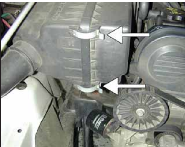
c. Unclip the two metal retaining clips on the air filter housing. Remove the air filter housing lid and air filter.
