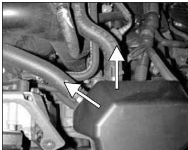
d. Pinch the two hose clamps and pull the breather hoses from the air box.
