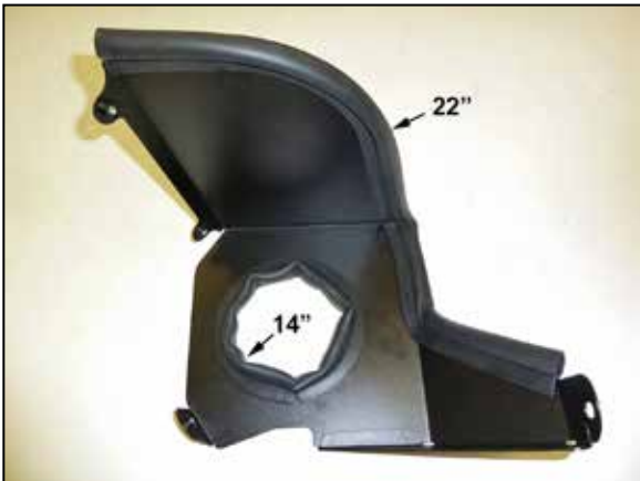
10. Install the 14" and 22" edge trim onto the heat shield as shown.
