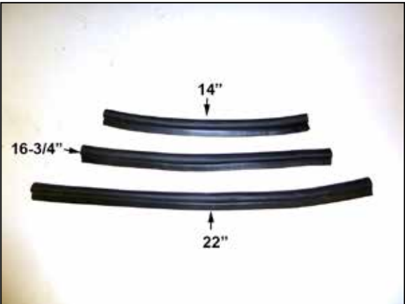
9. Cut the provided edge trim into sections of 14", 16-3/4", 22"
