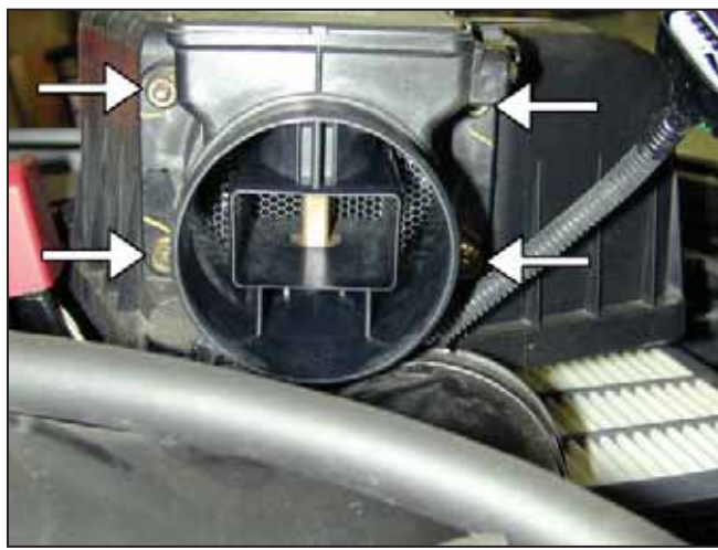
d. Loosen the four nuts that hold the MAF sensor to the airbox. Carefully set aside the MAF sensor.
