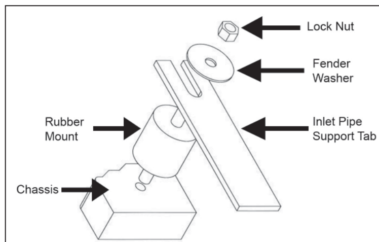
Proper rubber mount installation
