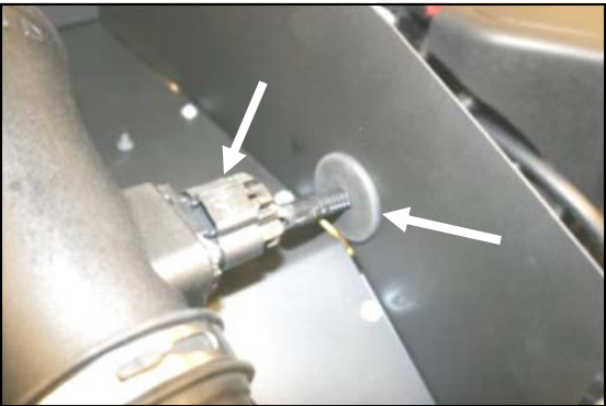
14. Re-connect the wiring connector to the MAF, and then seat the large grommet into the hole in the side of the CAD.
