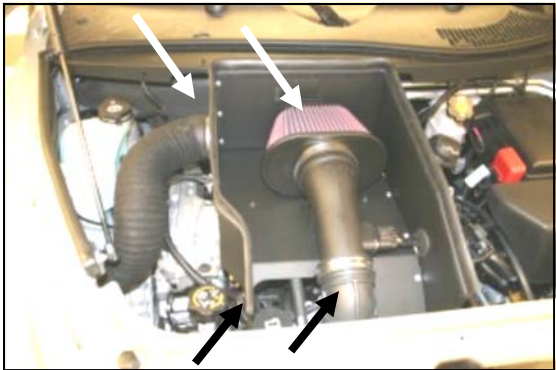
15. Install the Airaid Premium Filter (#1) onto the Airaid Intake Tube, and tighten the clamp. Install the weather strip (#6) on top of the CAD starting at the front corner, and working your way to the other corner. Reconnect the factory fresh air tube to the CAD, and tighten the hose clamp. Adjust the factory rubber elbow on the Airaid Intake Tube, and tighten the hose clamp.
