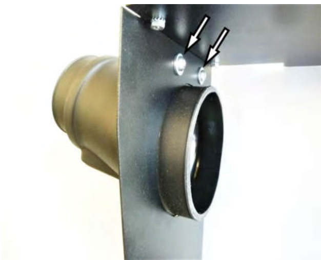
10. Mount the Sensor Tube onto the Panel Assembly and secure using the two 1/4-20 Button Head Screws and 1/4 inch Flat Washers.
