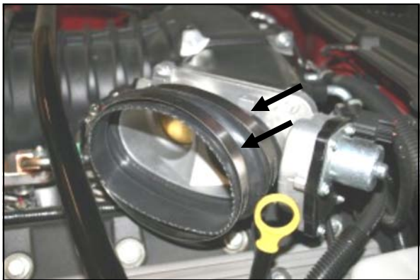
10. Install the oval hump hose (#4) onto the throttle body with two provided #80 hose clamps (#9). Leave the clamps loose for now.
