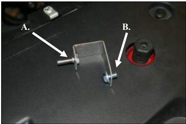
10.A.) Thread the 1/4-20 hex bolt (#13) into the resonator bracket (#21) and tighten as shown. B.) Slide the 6mmx12mm (#15) hex bolt thru one flat washer (#11) and into the hole in the resonator bracket.
