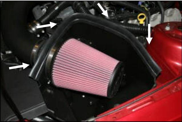
14. Install the Airaid Premium Filter (#1) onto the filter adapter and tighten the hose clamp. Next, install the weatherstrip (#9) onto the top of the CAD as shown starting near the radiator and working your way towards the left fender.
