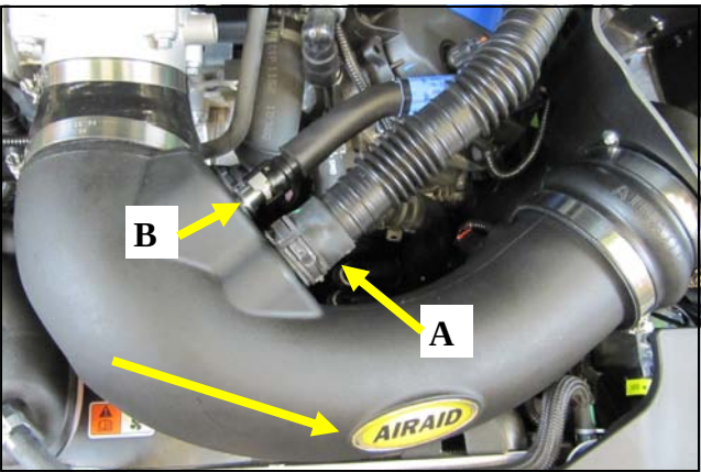
11. Install the Airaid Intake Tube into the couplers as shown, and tighten all Hose Clamps. A) Reconnect the Resonator tube to the Airaid Intake using the OEM clamp. B) Reconnect the breather line/lines to the Aluminum Fittings depending on your application. Apply the Airaid Decal onto the Tube as shown.
