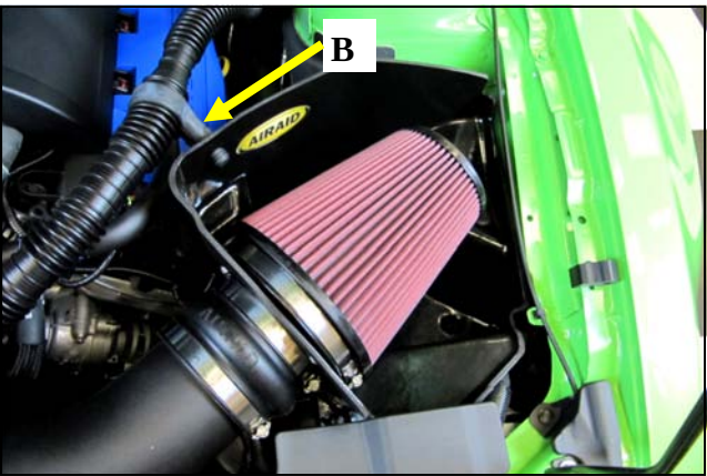
12. A) Install the Airaid Premium Filter onto the filter adapter and tighten the hose clamp. B) re install the Resonator tubing into the factory Stand off.
