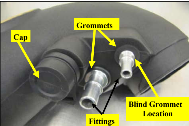
17. Insert the remaining 1/2" and 13/16" Grommets with Aluminum Fittings into the Airaid Intake tube as shown. Install the resonator Cap and secure it using the Speed clamp. On vehicles not equipped with the small breather, plug the hole with the Blind Grommet.
