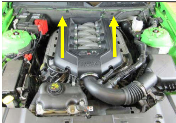
2. Lift straight up on the engine cover to unseat it from the mounting grommets and set it aside.
