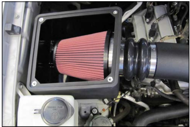
13. Install the Airaid Premium Filter onto the Filter Adapter inside of the airbox and tighten the clamp..
