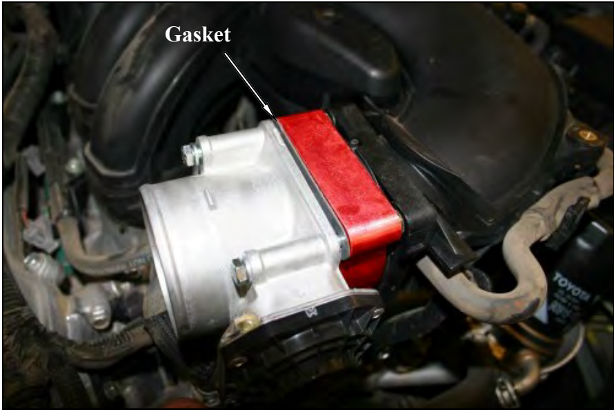
6. Slide the Airaid Spacer (#1) and gasket (#2) between the intake manifold and the throttle body. Make sure the “Flow” arrow on the spacer is pointing towards the intake manifold, and the gasket is next to the throttle body. Install the 4 supplied 6mm x 75mm bolts (#3) and flat washers (#4) thru the throttle body, gasket, spacer, into the intake manifold and tighten evenly to the vehicle manufacturer’s specifications.
