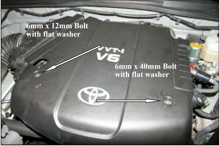
10. Gently reinstall the beauty cover on the engine and use one 6mm x 12mm bolt (#8) with flat washer (#4) on the passenger side, and one 6mm x 40mm bolt (#7) with flat washer (#4) on the driver’s side.
