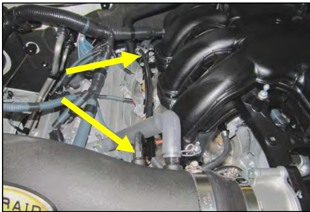
12. Connect the factory crank case breather line to the 3/8 Barbed Fitting on the Intake Tube and replace the OEM vacuum line on the fuel pressure regulator with the supplied 17' 1/8" line. Connect the 1/8" line to the second Fitting on the Intake tube.
