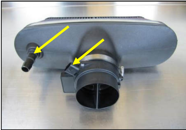
5. Transfer the Mass Air Flow meter into the Airaid Filter Assembly. Note the positioning of the air meter socket in relation to the breather coupling.
