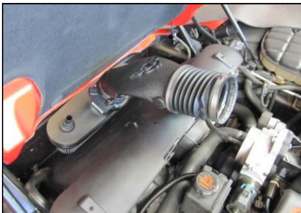
7. Reinstall the OEM intake tube onto the MAF and Filter Assembly then lower into the inner bumper area. When properly installed the Filter end cap will positively engage the grommet posts on the inner frame.
