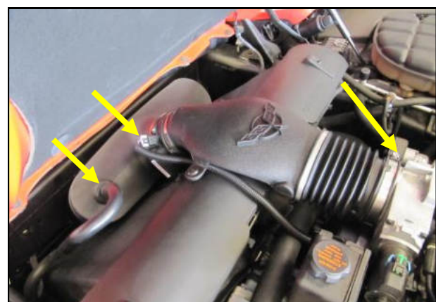
8. Re-secure the intake tube onto the throttle body and re seat the grommets on the radiator shroud posts. Re connect the MAF and air pump breather line.
