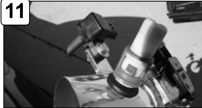
Install VSV valve to bracket on tube and secure using screw, flat washer, wavy washer and nut. Tighten using 10mm socket and wrench. Attach plastic fitting from step 4 to grommet on tube.
